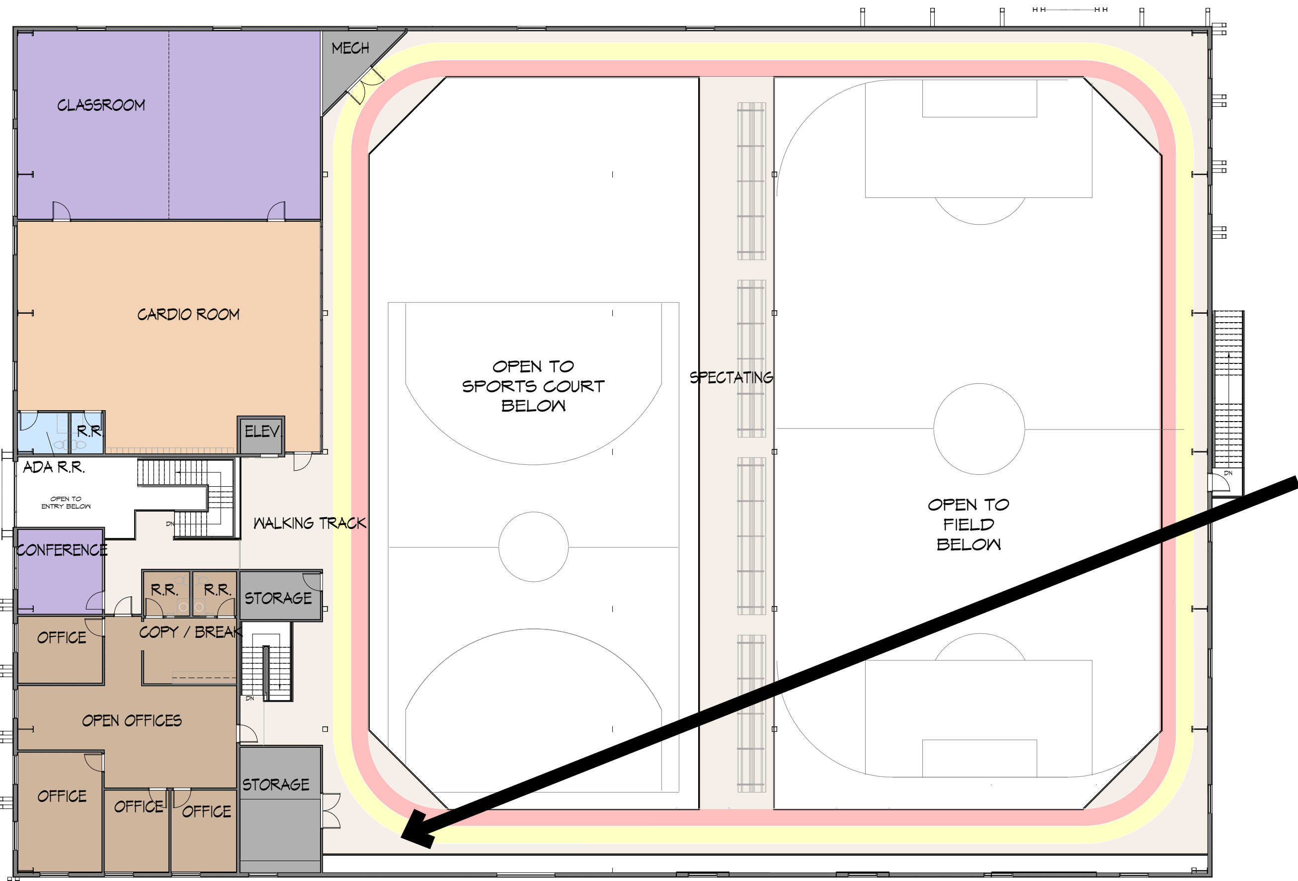
1/10 OF A MILE WALKING TRACK
